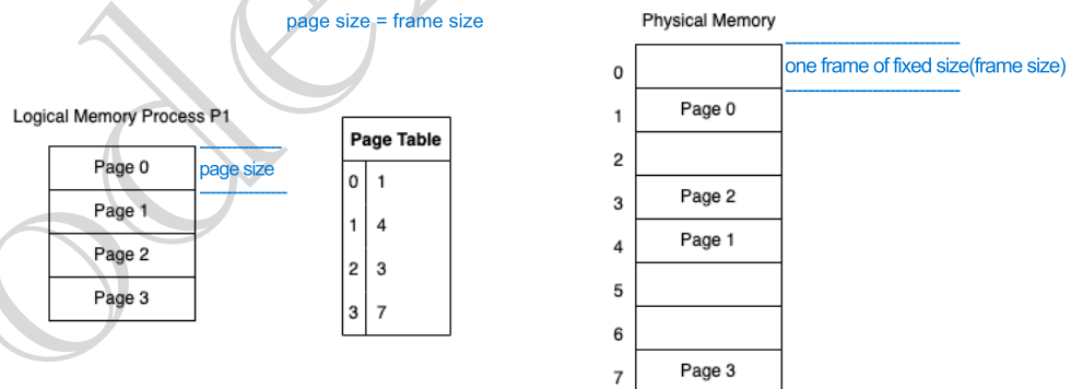
Paging model of logical and physical memory
